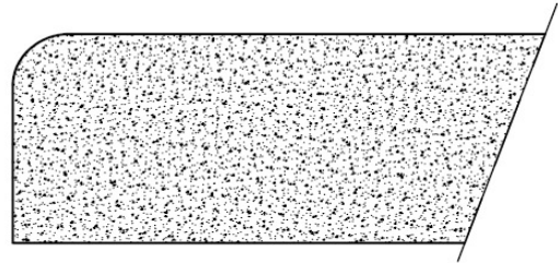
\frac{3}{8} " ROUND
